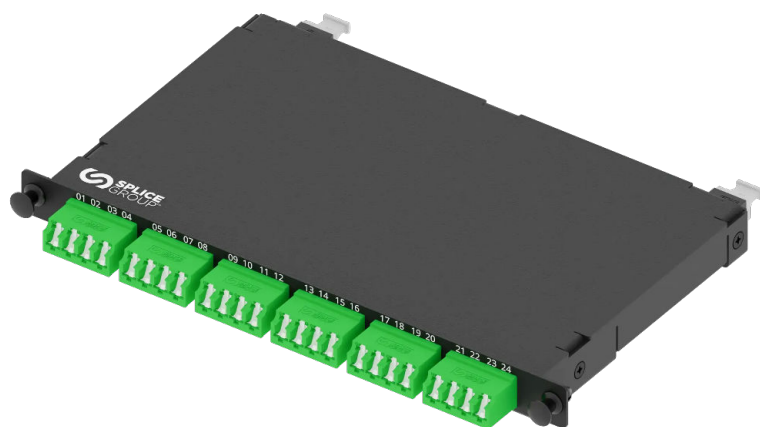
2x 12 Fibre MTP®/MPO - LCAPC
