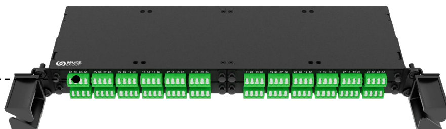
Modules Installed in 1U 19" 4-Way HD Customer Termination Panel
